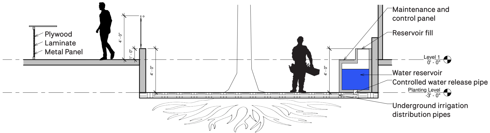
Circulation Section - NTS
